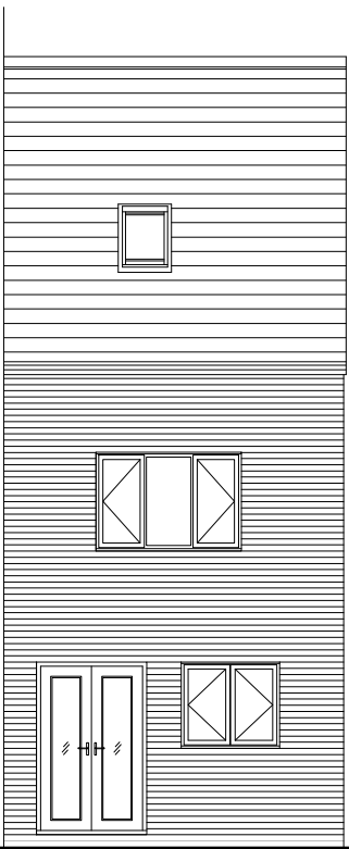
Rear Elevation
