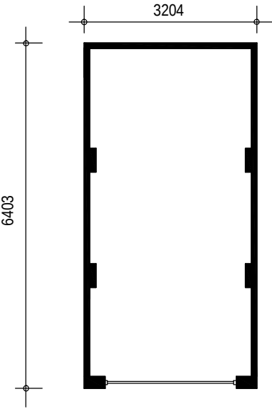
Floor Plan
