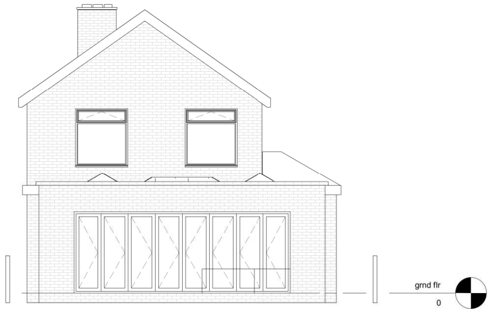
Proposed Elevation-Rear
