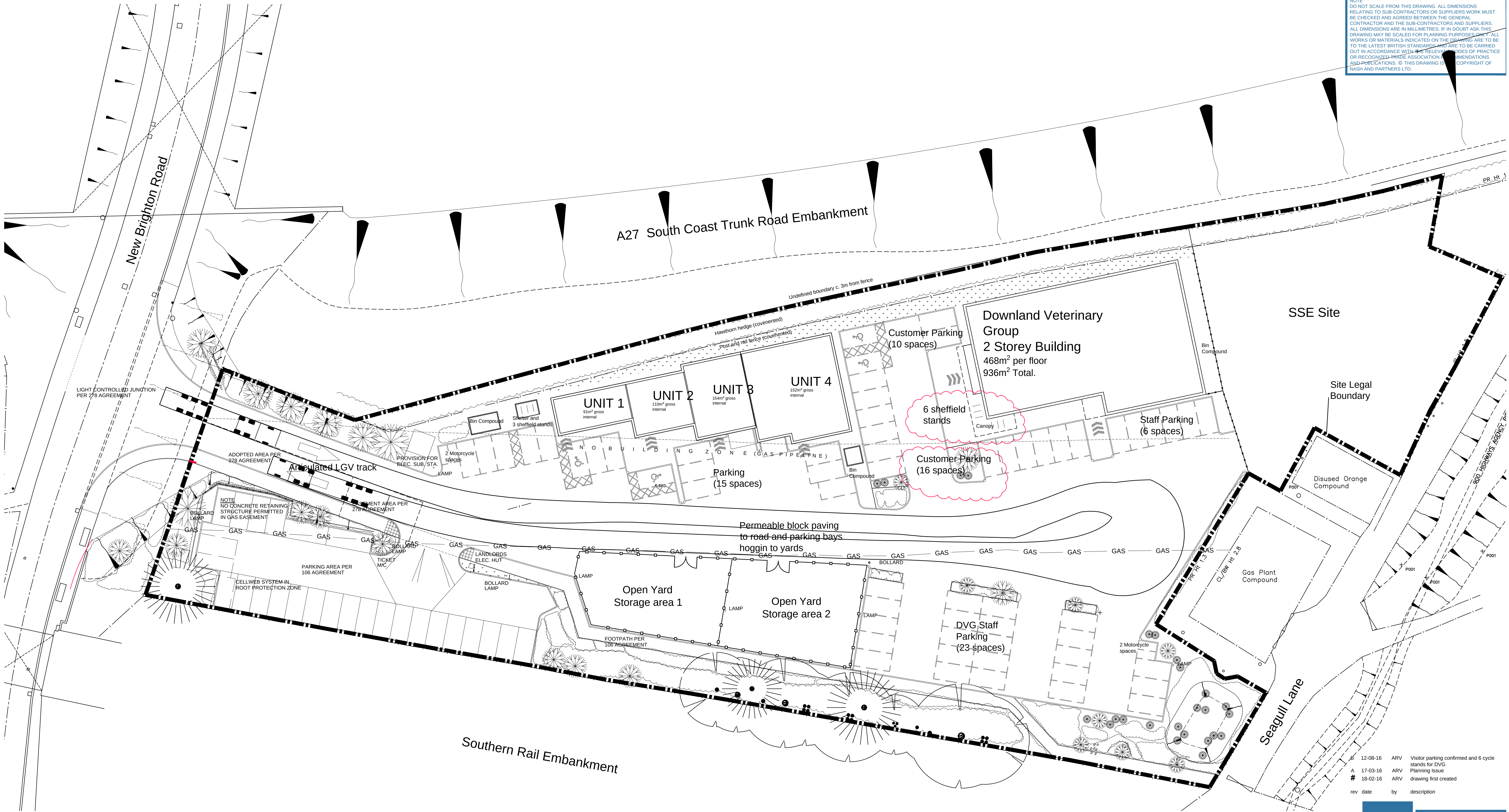
SITE LAYOUT PLAN (Scale 1:250)
