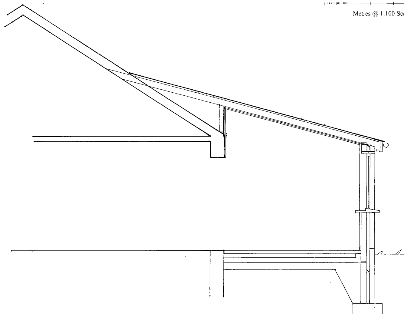
Cross-Section
