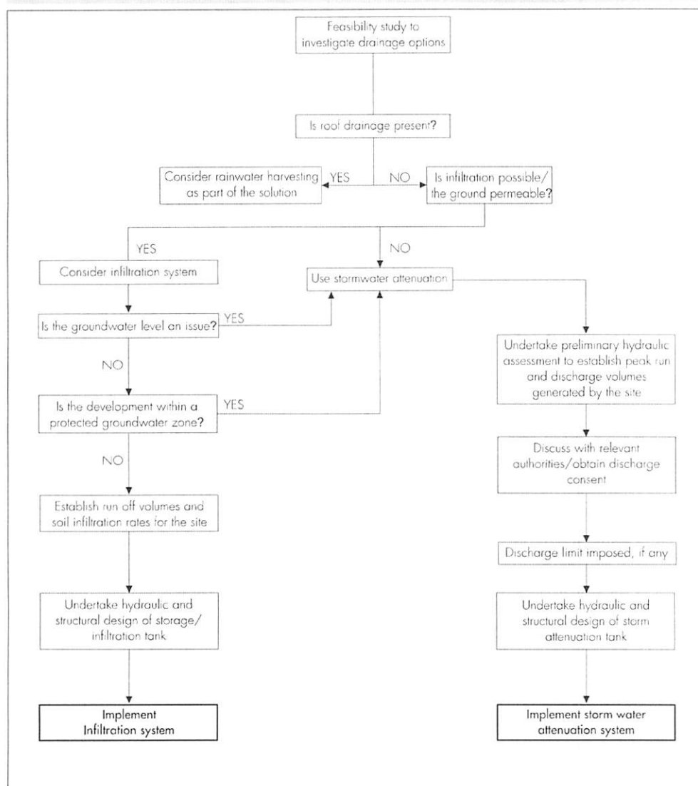
Figure 2 Sustainable drainage system selection and design
