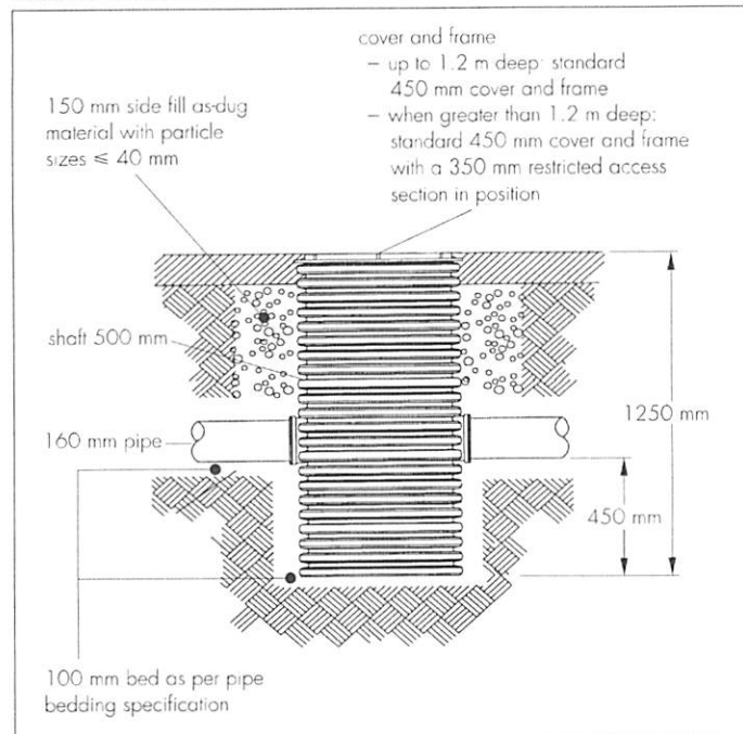
Figure 5 Typical silt trap
