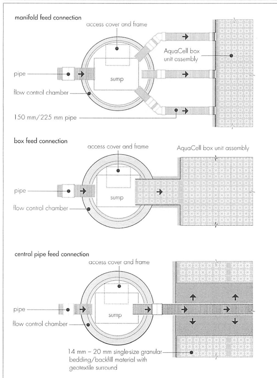
Figure 3 Typical inlet connection designs
