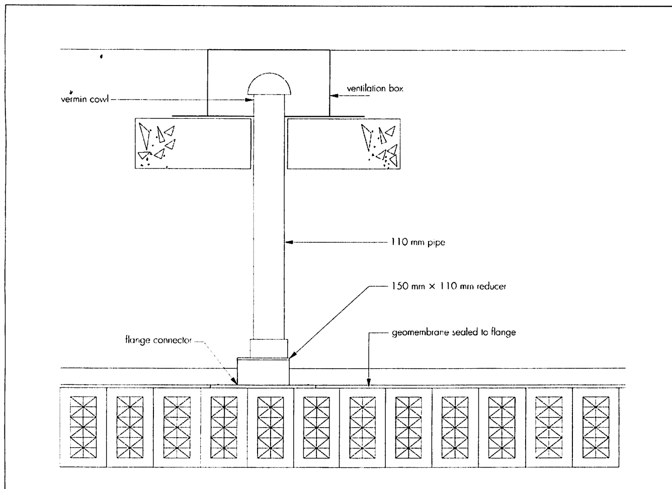
Figure 4 Typical air vent system
