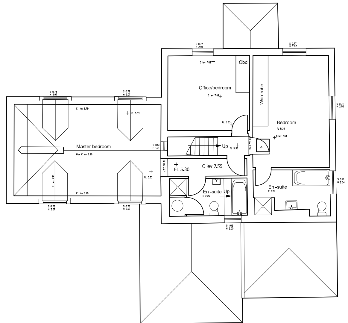
First floor
