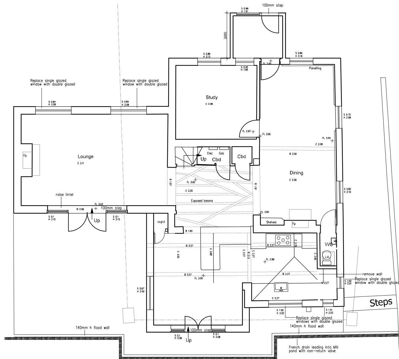
Ground floor
