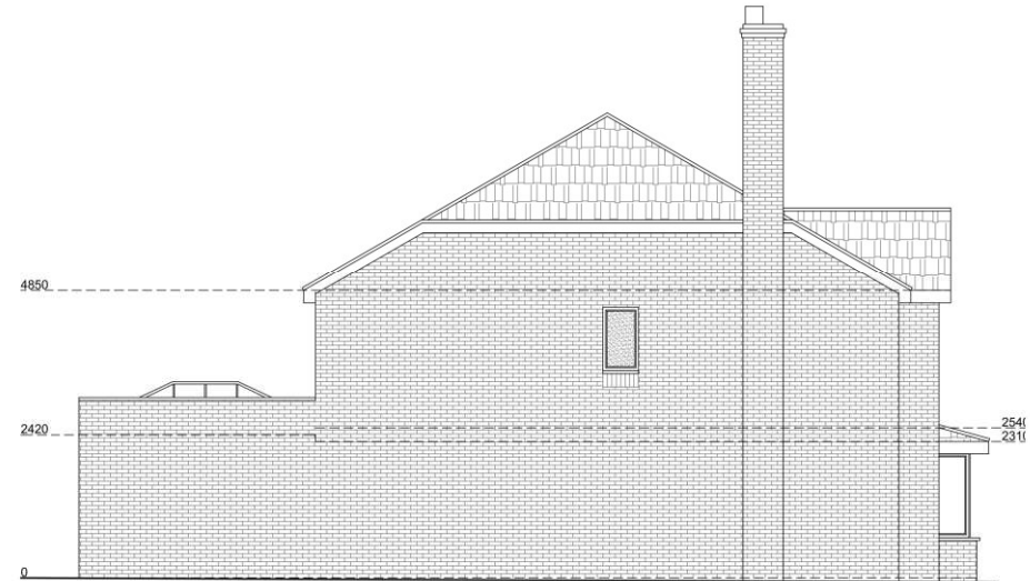
Proposed East Elevation Scale 1:50
