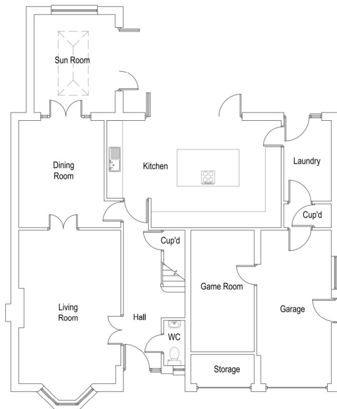
Existing Ground Floor Plan Scale 1:50
