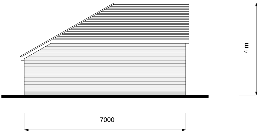
Proposed South West Elevation at 1:100 scale
