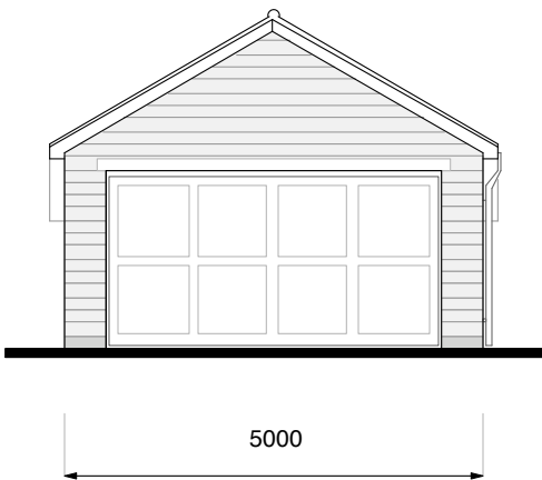
Proposed South East Elevation at 1:100 scale
