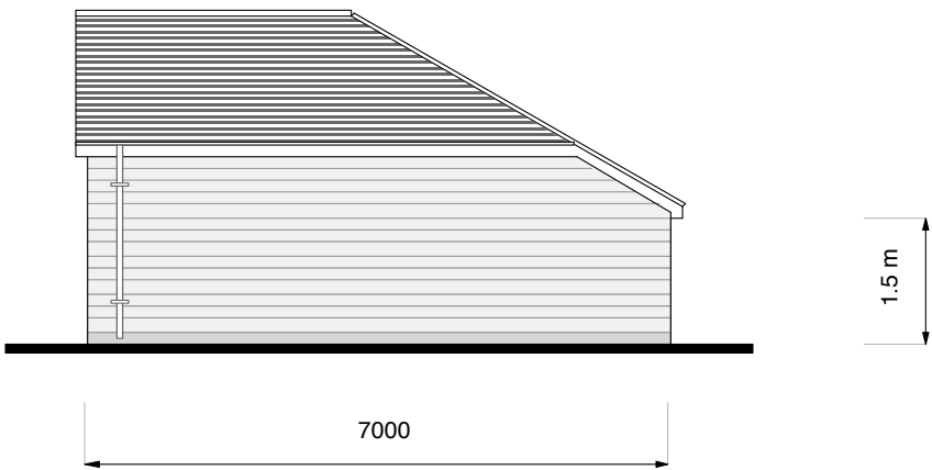
Proposed North East Elevation at 1:100 scale
