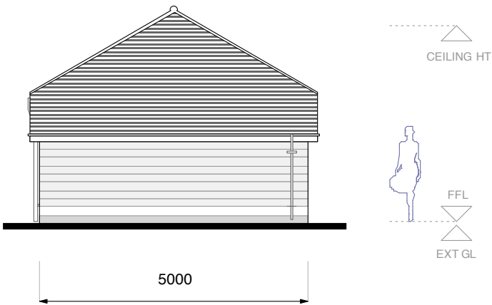
Proposed North West Elevation at 1:100 scale
