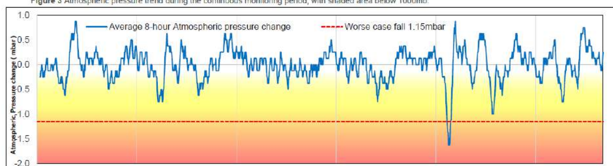
Figure 4 8-hour average atmospheric pressure trend during the continuous monitoring period.
