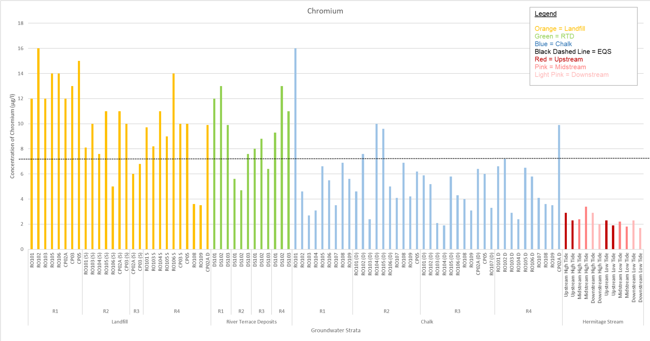
Diagram 5 – Chromium Concentrations in Groundwater and Hermitage Stream
