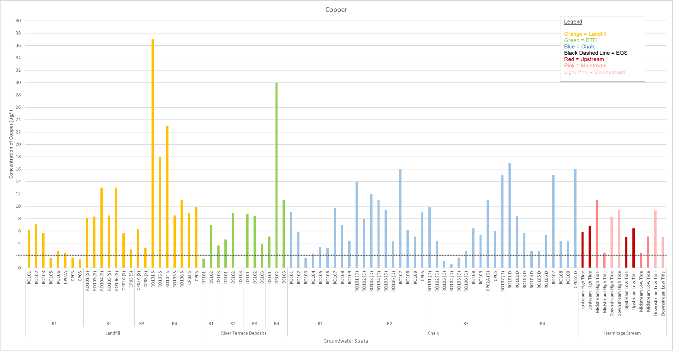
Diagram 6 – Copper Concentrations in Groundwater and Hermitage Stream
