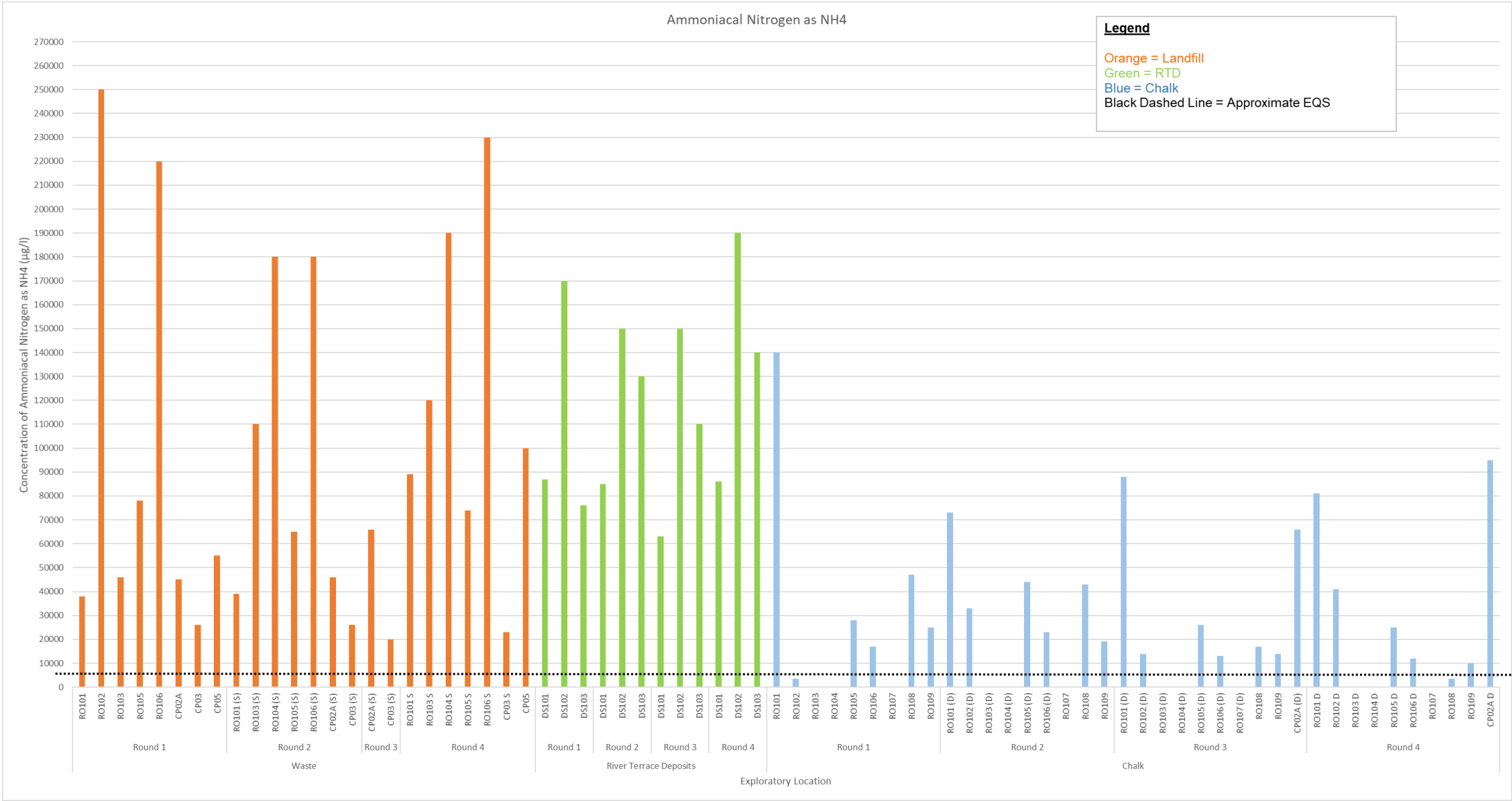
Diagram 9 – Ammoniacal Nitrogen as NH4 Concentrations in Groundwater
