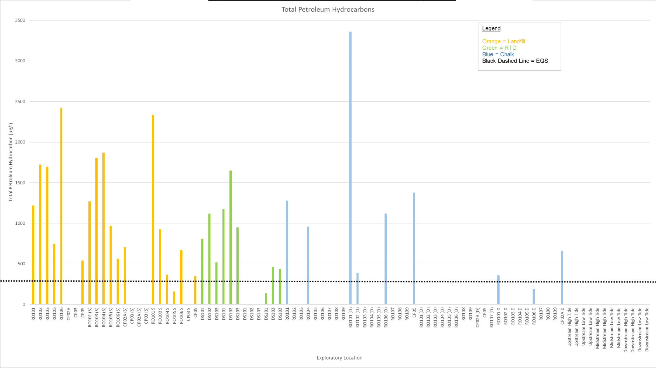
Diagram 11 – TPH Concentrations in Groundwater and Hermitage Stream
