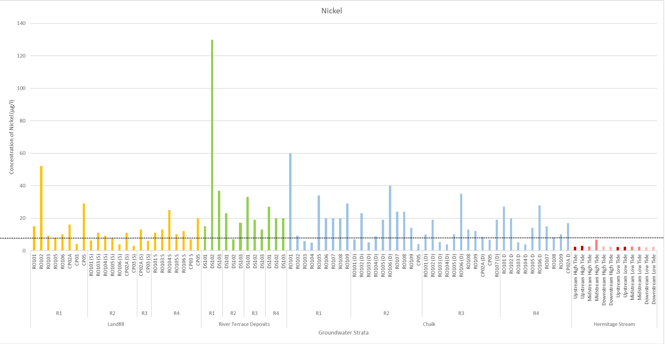
Diagram 7 – Nickel Concentrations in Groundwater and Hermitage Stream
