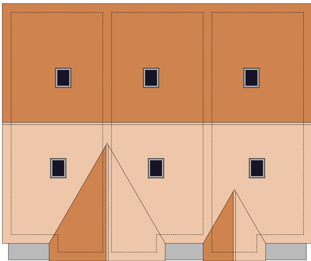
ROOF PLAN
