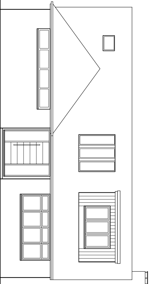
South (front) 1:100
