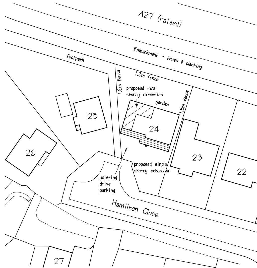
Site Plan 1 to 500
