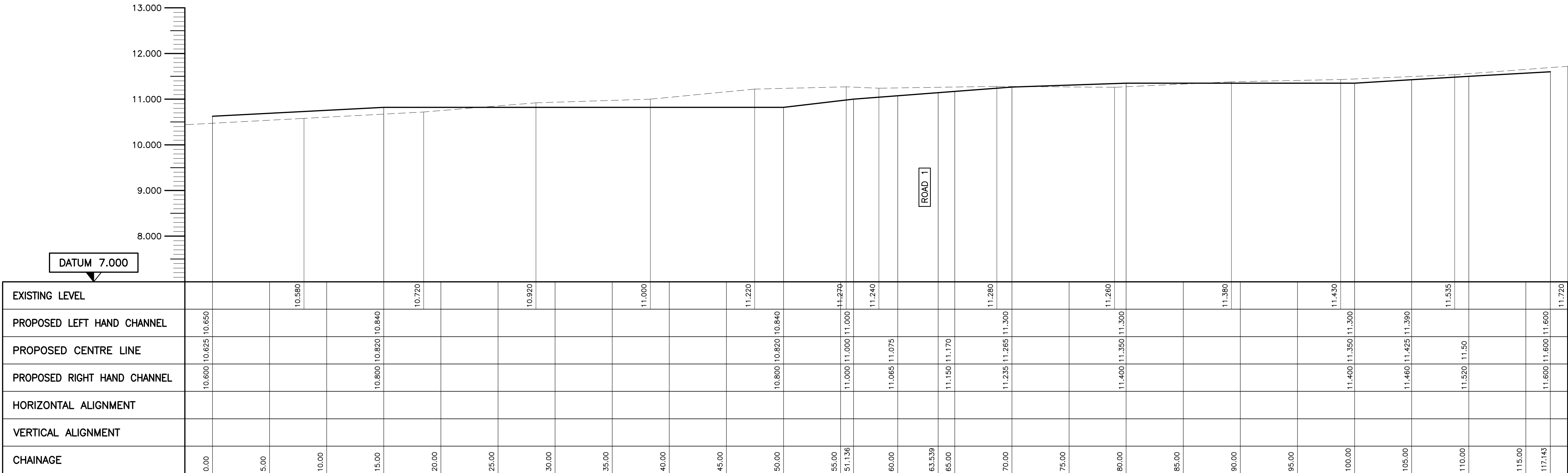
ROAD 2 LONG SECTION (SCALE: HORIZONTAL 1:200, VERTICAL 1:50@A1)
