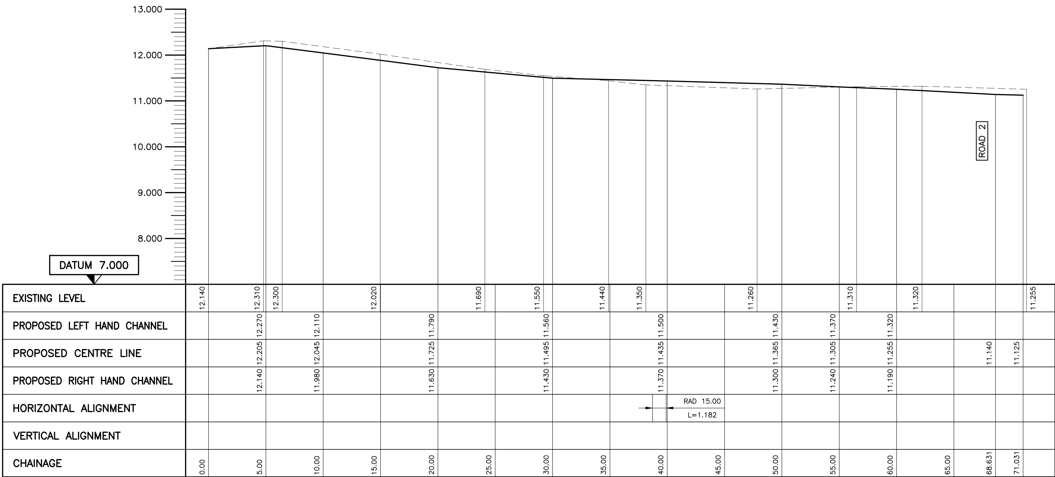
ROAD 2 LONG SECTION (SCALE: HORIZONTAL 1:200, VERTICAL 1:50@A1)
