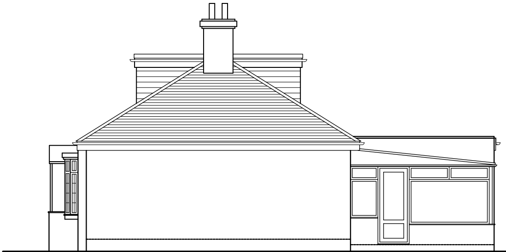
NORTH ELEVATION
