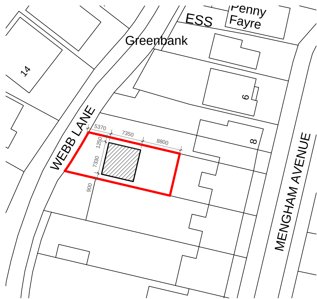
BLOCK PLAN 1:500
