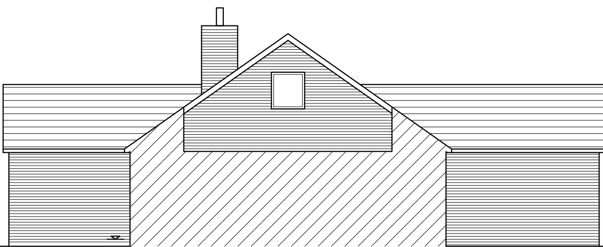
EXISTING WEST ELEVATION scale 1_100
