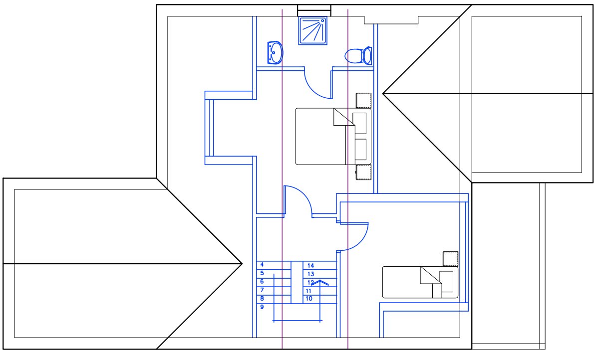
PROPOSED ATTIC scale 1_100
