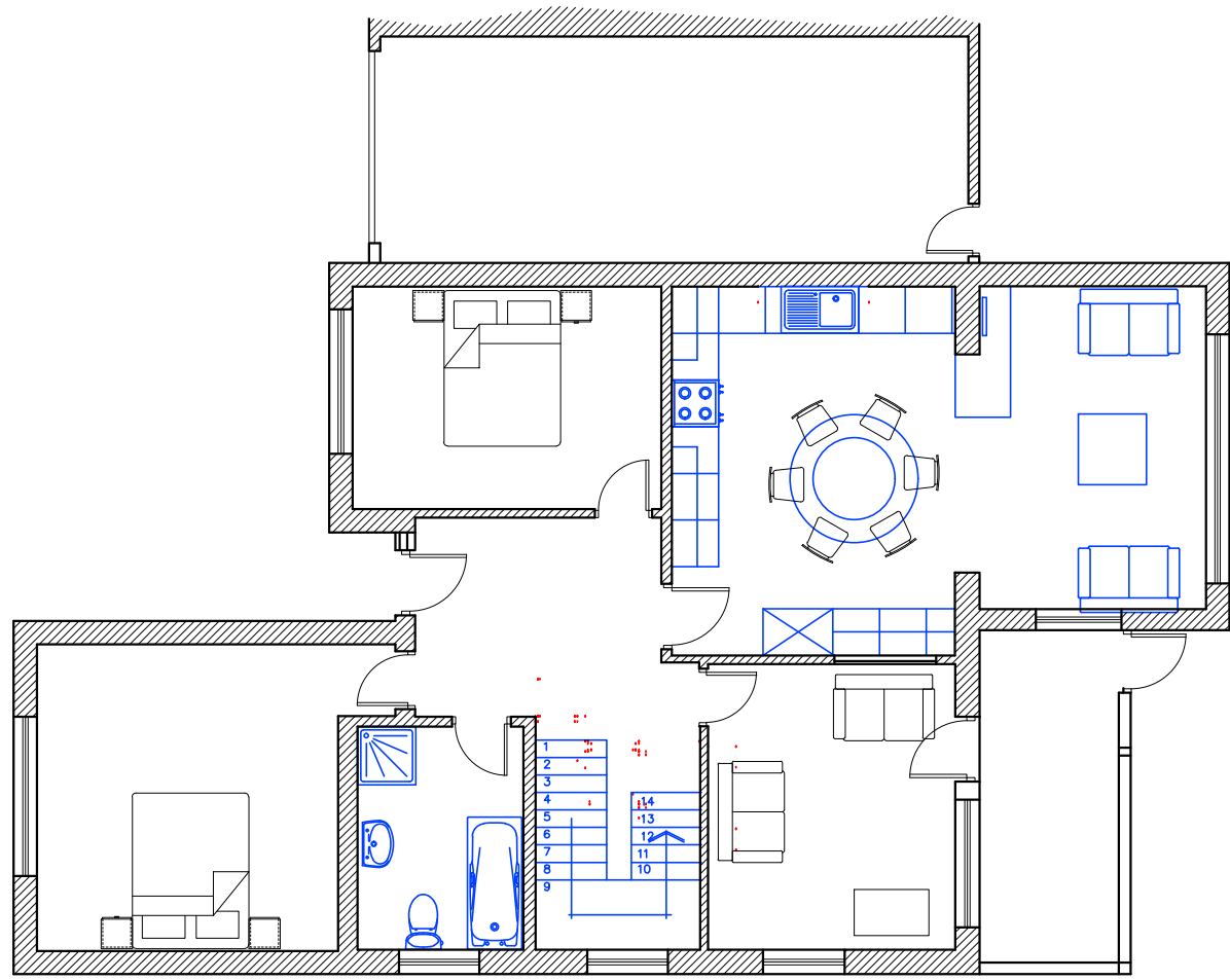
PROPOSED GROUND FLOOR [1] scale 1_100
