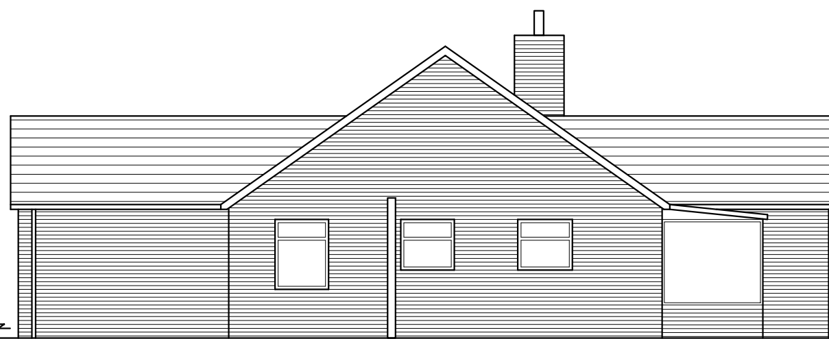
EXISTING EAST ELEVATION scale 1_100
