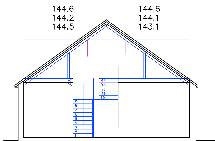
PROPOSED SECTION scale 1_100
