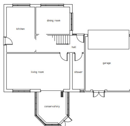
GROUND FLOOR LAYOUT PLAN
