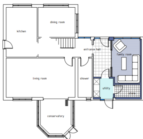
GROUND FLOOR LAYOUT PLAN
