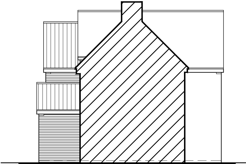
SOUTH FACING PROPOSED FRONT PORCH
