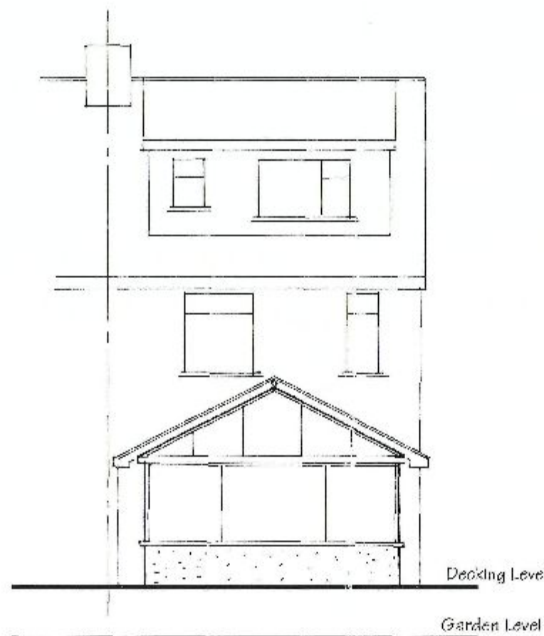
Proposed West/Rear Elevation
