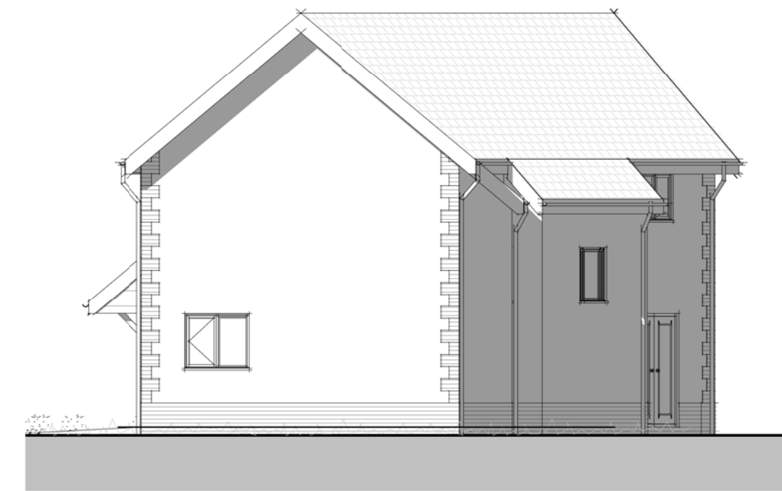
Side Elevation B 1 : 100
