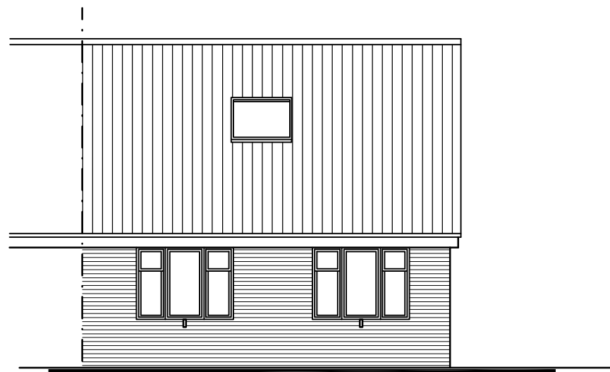
SOUTH ELEVATION
