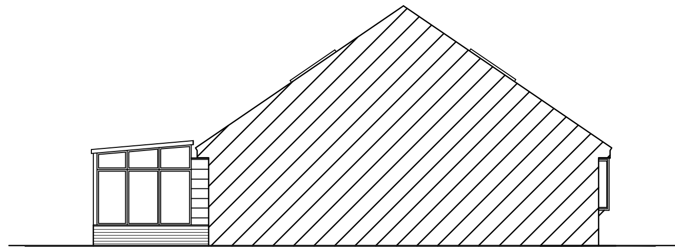
WEST ELEVATION
