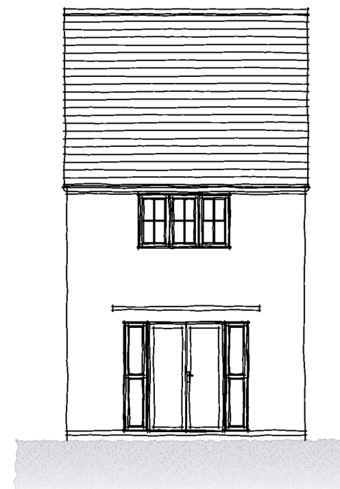
REAR ELEVATION
