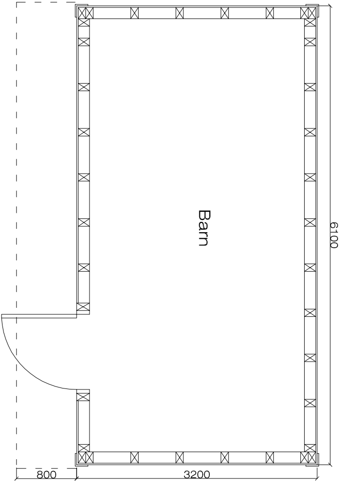
Floor Plan
