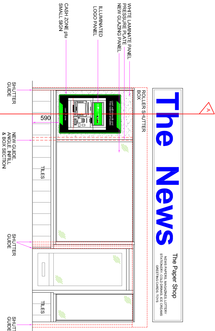
PROPOSED (PART) PLAN
