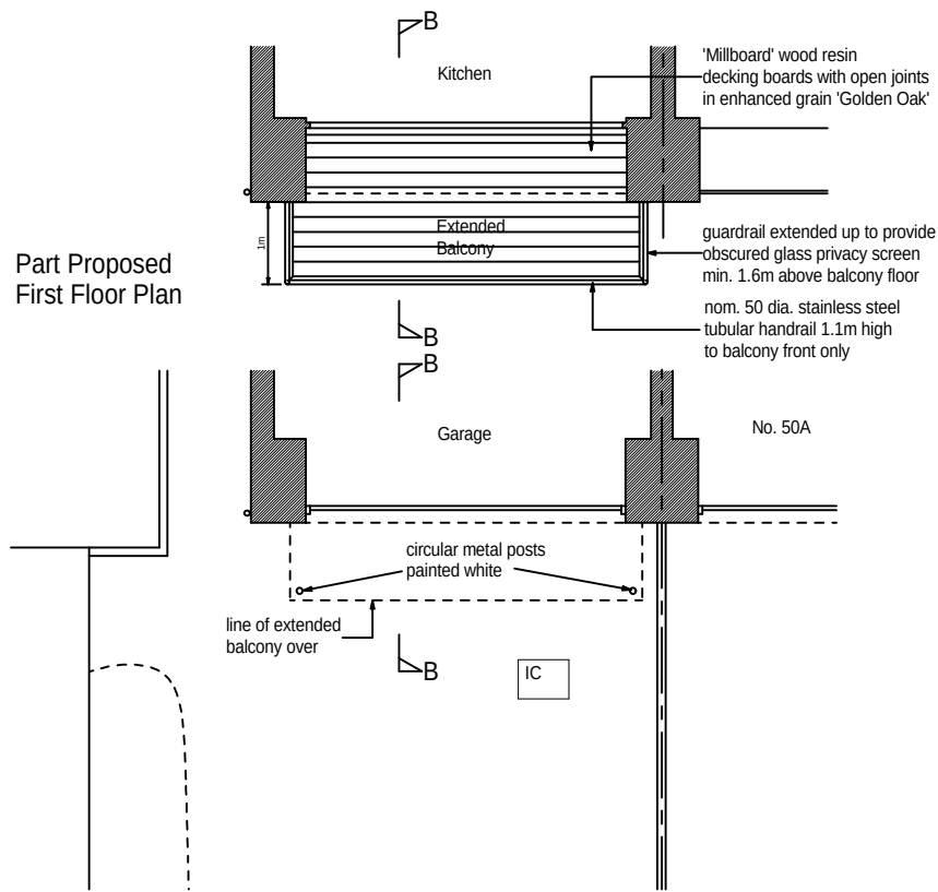
Part Proposed First Floor Plan 1:100
