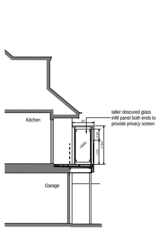
Proposed Section B-B
