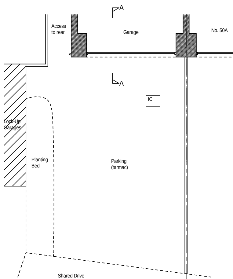
Part Existing Ground Floor & Site Plan 1:100
