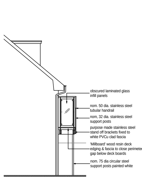
Part Proposed Side Elevation (North)
