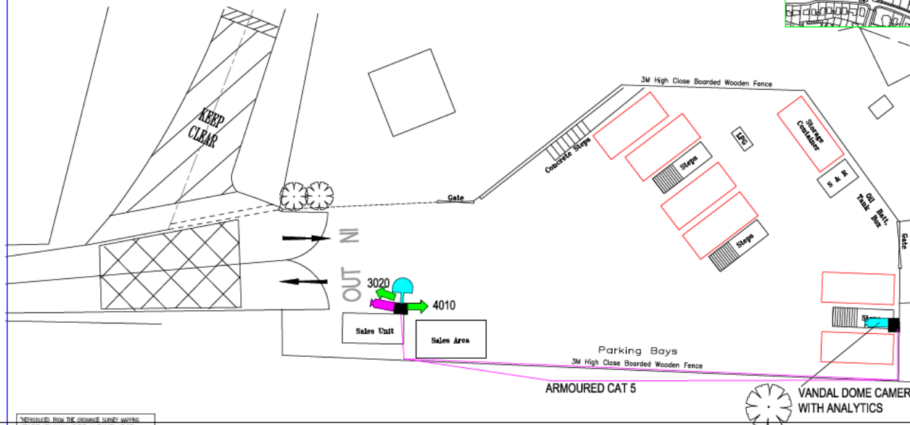
PLAN SCALE 1/250
