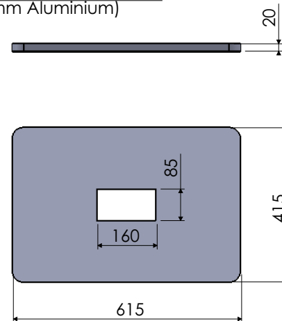
Baseplate Cover Shroud (2.5mm Aluminium)
