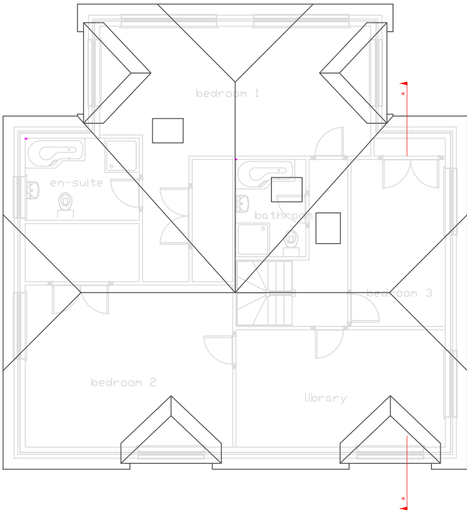
ROOF PLAN EXISTING
