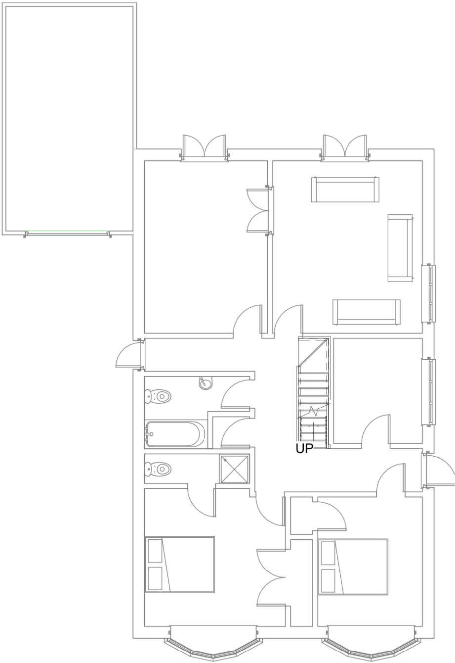
1 Ground 1 : 100
