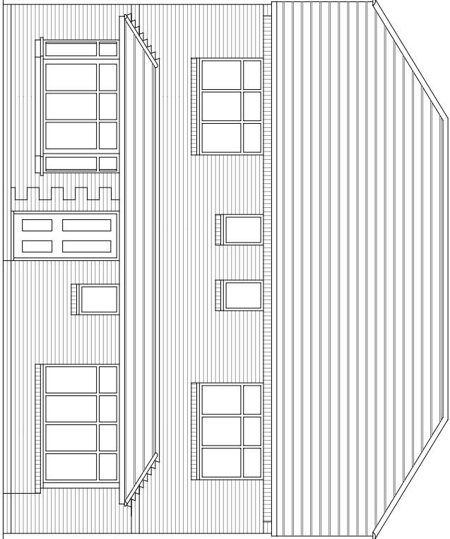
existing front (south) elevation
