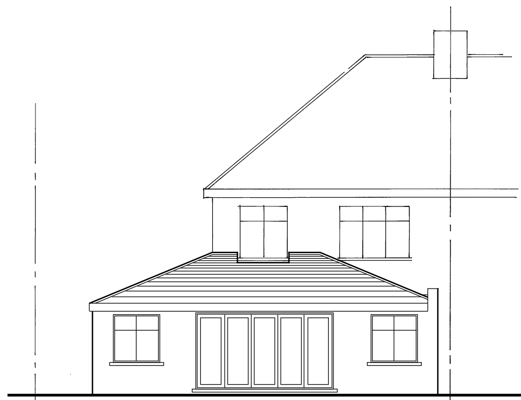
Proposed NW/Rear Elevation
