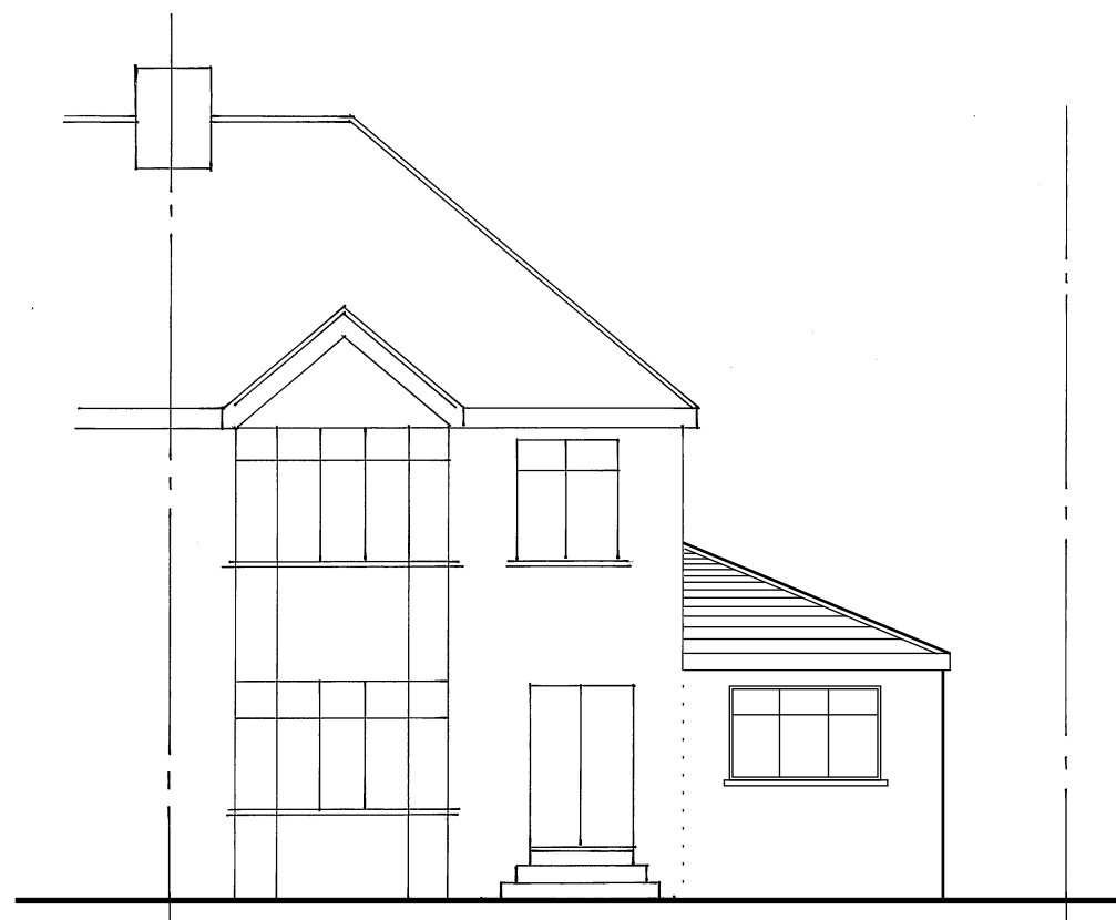
Proposed SE/Front Elevation
