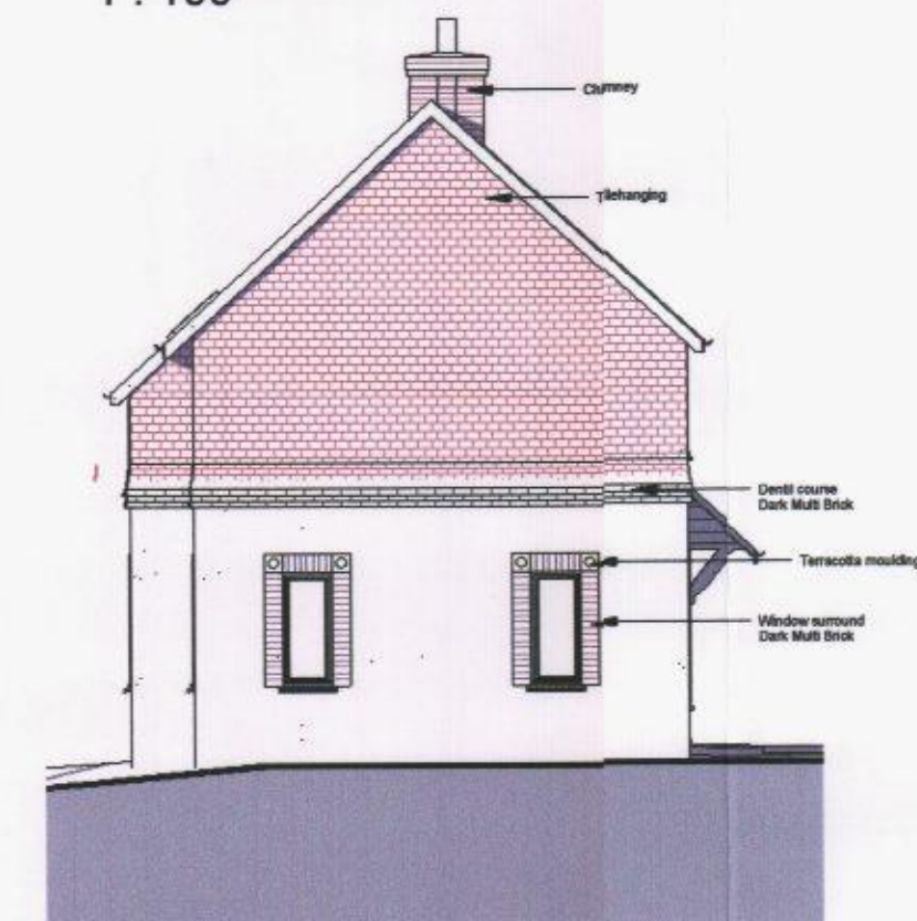
Type 20- Plot 17 Front Elevation 1 : 100
