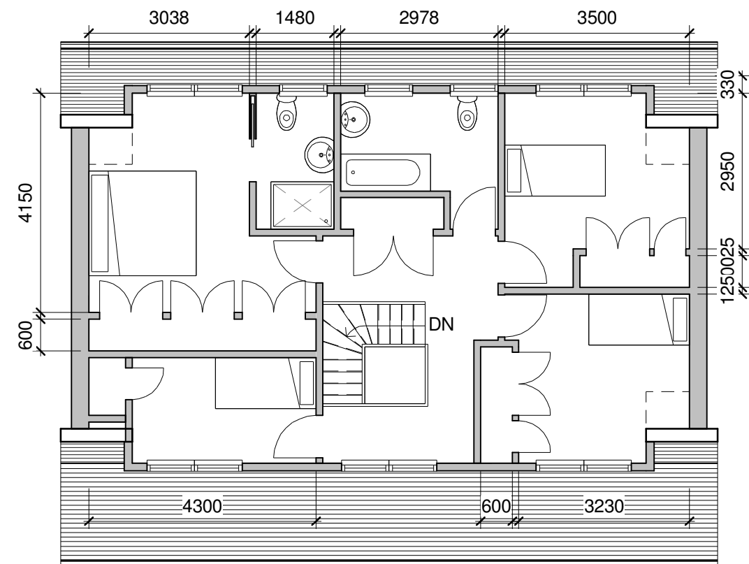
Proposed First Floor 1 : 100
