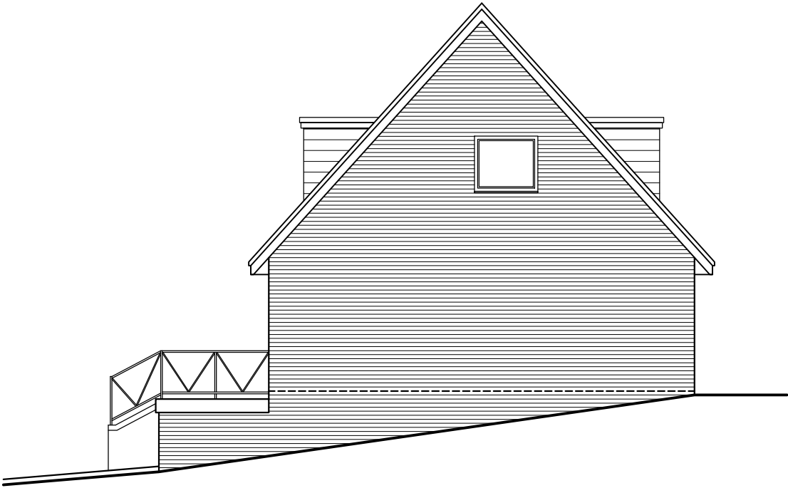
1:100 SIDE (SOUTH)ELEVATION
