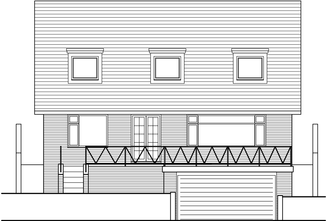
1:100 FRONT (WEST)ELEVATION
