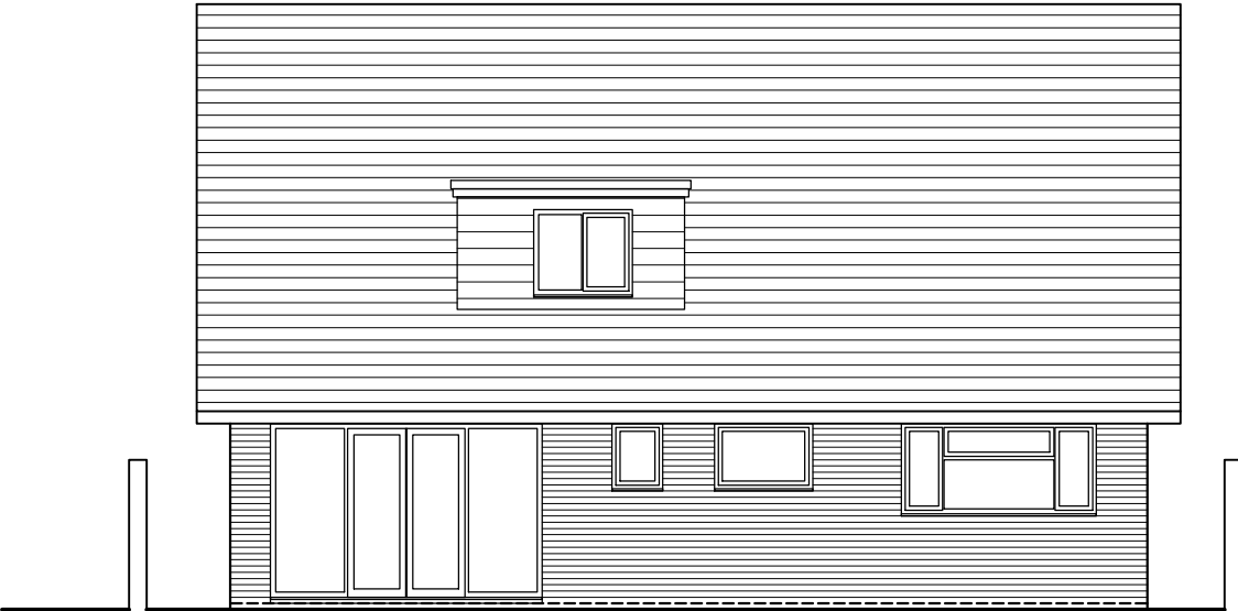
1:100 REAR (EAST)ELEVATION
