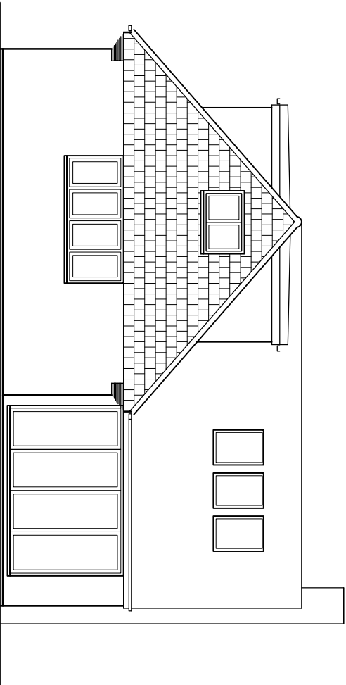
Rear (north) 1:100
