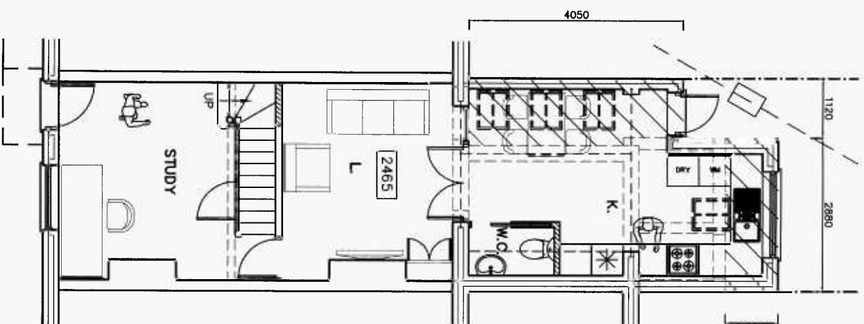
GROUND
