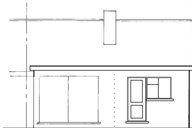
Proposed South/Rear Elevation
