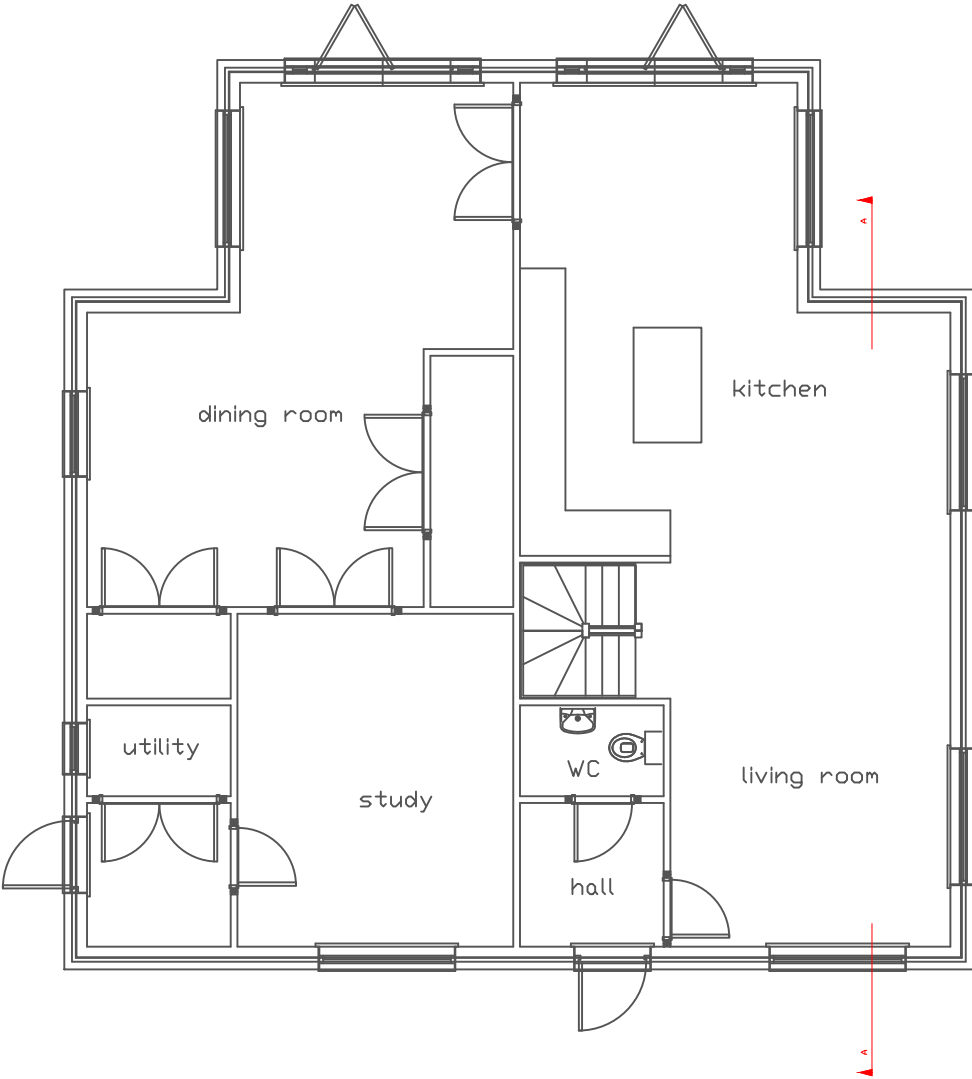
GROUND FLOOR PLAN EXISTING
