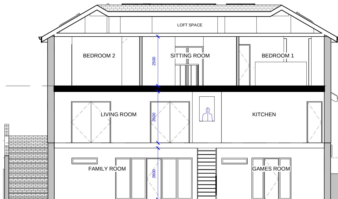
SECTION C-C
