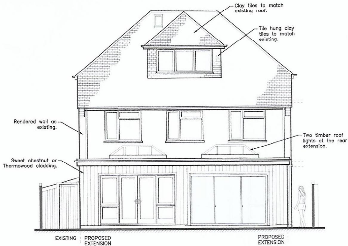
PROPOSED SOUTH ELEVATION REF. NO.: 27-S
