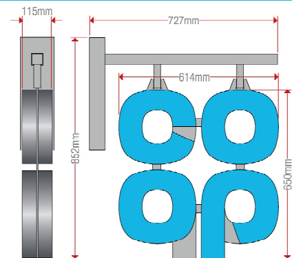
Size 2 - 650mm Scale 1:10
