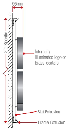
Logo Cross Section Scale 1:10 @A3
