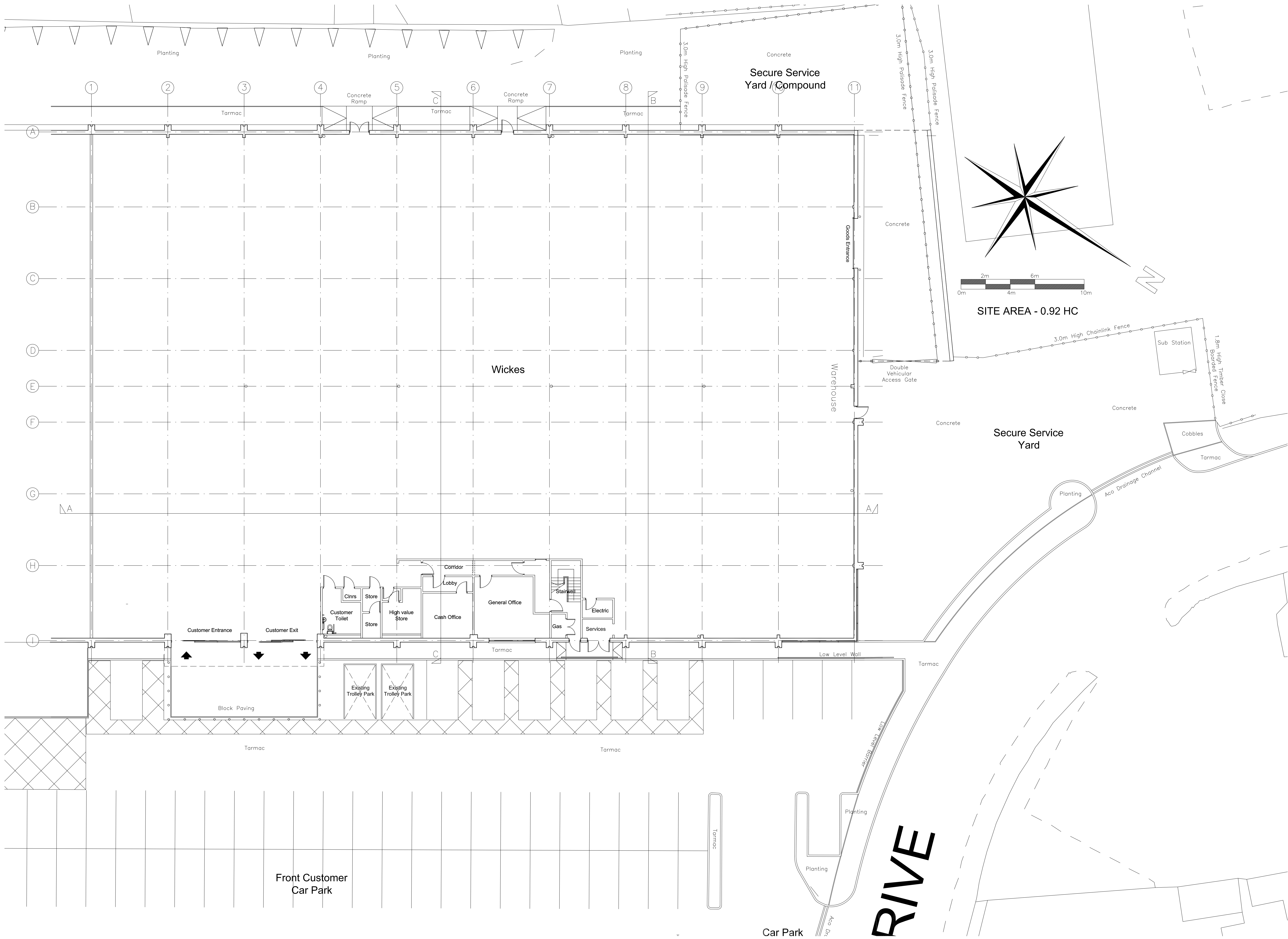
Existing Site Layout (1:100)
