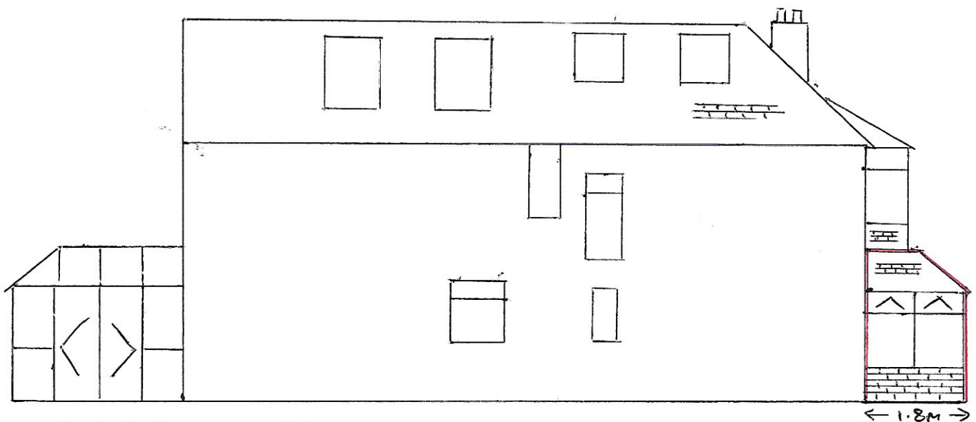
LH Side Elevation - Proposed
