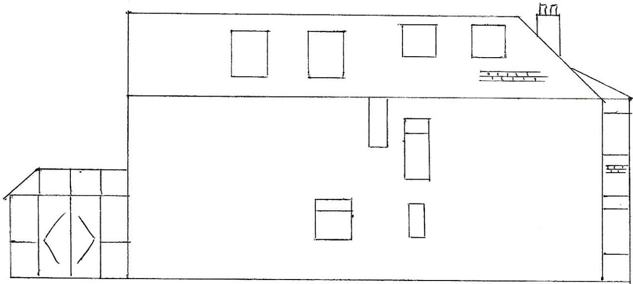
LH Side Elevation - Existing
