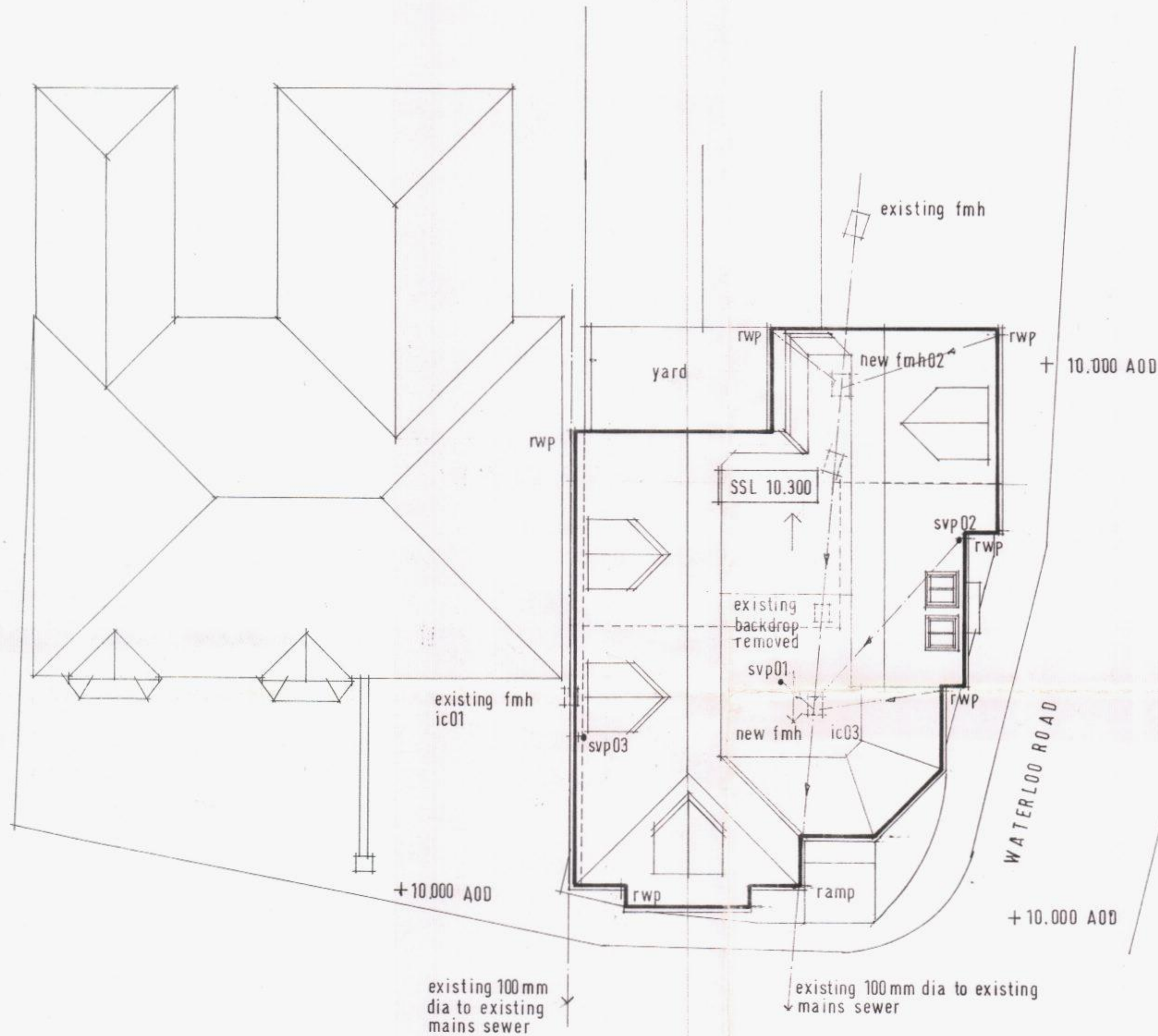
PROPOSED SITE / BLOCK PLAN SCALE 1:50
