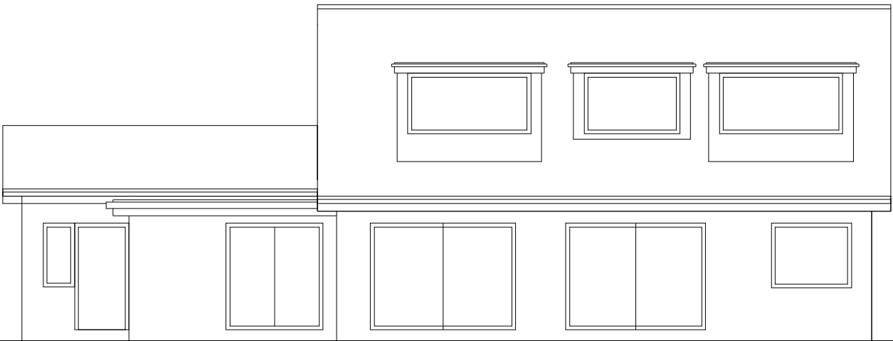
Rear Elevation | Existing
