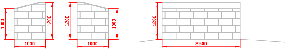
COMPOSTER BOX ELEVATIONS
