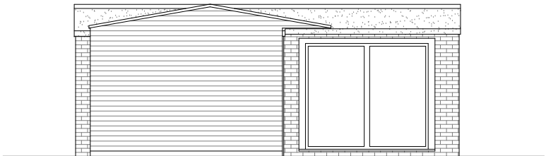
SIDE ELEVATION
