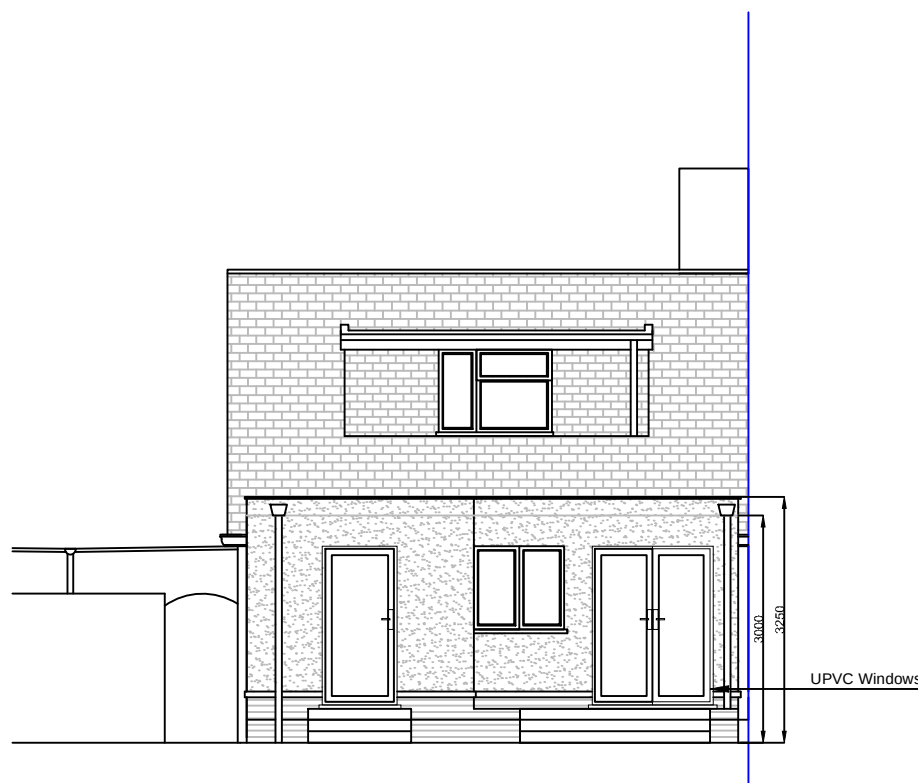
Rear Elevation
